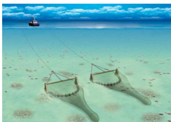
Figure 3-11 Typical beam trawler and gear diagram (Source: Seafish, 2015; Hook and Net Magazine, 2020)
