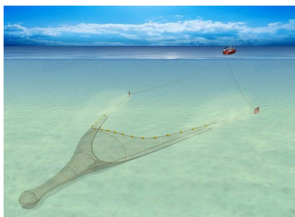
Figure 3-12 Typical otter trawler and gear diagram (Source: Seafish, 2015, MarineTraffic, 2022)
